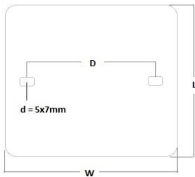
Faceplate
